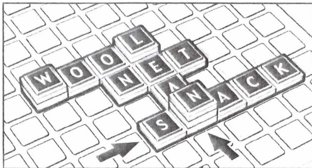
Figure 6 Score: 14 Points
